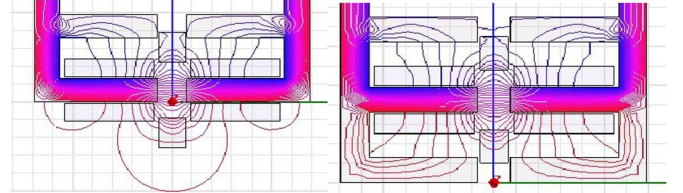
Fig. 4. Magnetic flux distribution of (left) phase A and (right) phase B.
