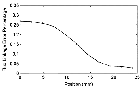
Fig. 9. Percentage variation of flux linkage error with translator position.
