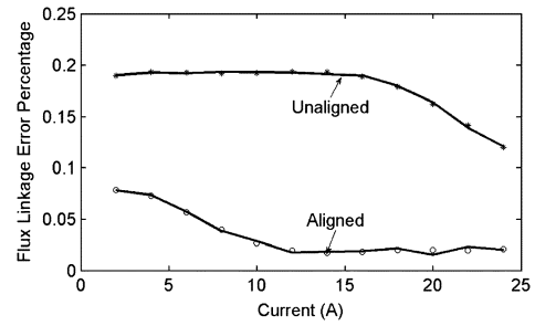
Fig. 8. Percentage variation of flux linkage error with excitation current.
