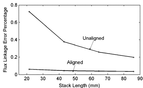
Fig. 10. Percentage variation of flux linkage error with stack length.
