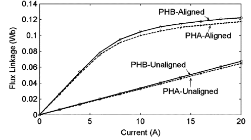
Fig. 3. Flux linkage comparison of phases A and B.
