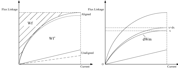
Fig. 2. Energy conversion procedure.
