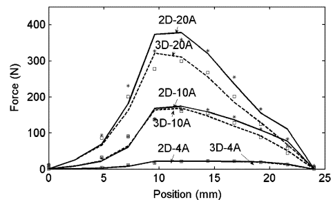
Fig. 12. Static force comparison of 2-D and 3-D FEA.
