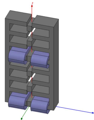
Fig. 1. Double-side LSRM.
