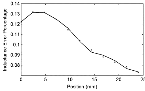
Fig. 6. Percentage variation of inductance error with translator position.
