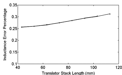
Fig. 11. Percentage variation of inductance error with translator stack length.
