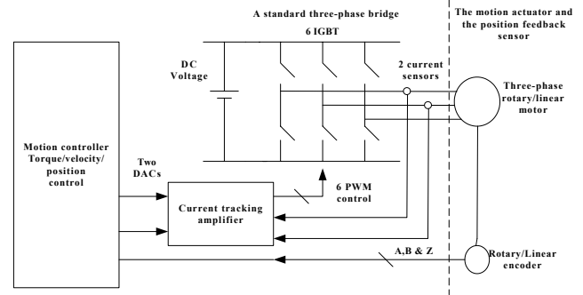
Fig. 1. Block diagram of a general-purpose three-phase motor controller.
