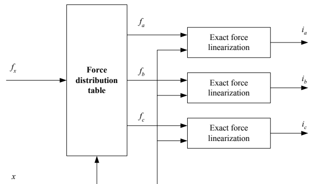
Fig. 3. Two-stage force linearization scheme.
