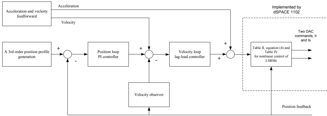
Fig. 6. Motion controller for the proposed system.
