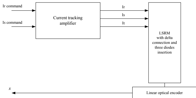
Fig. 5. Amplifier and LSRM setup.
