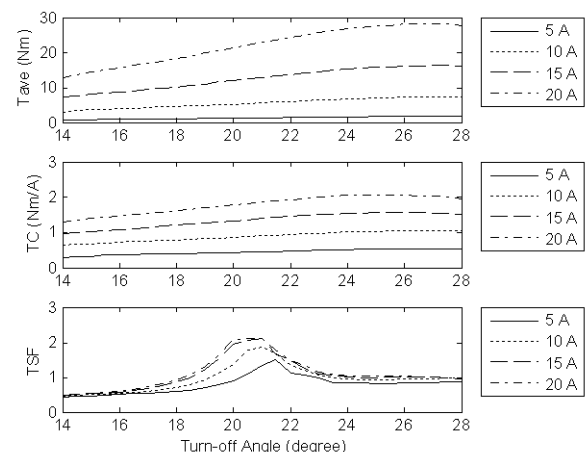
(b) Various current references
