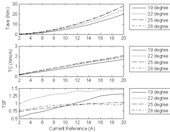
(b) Various turn-off angles
