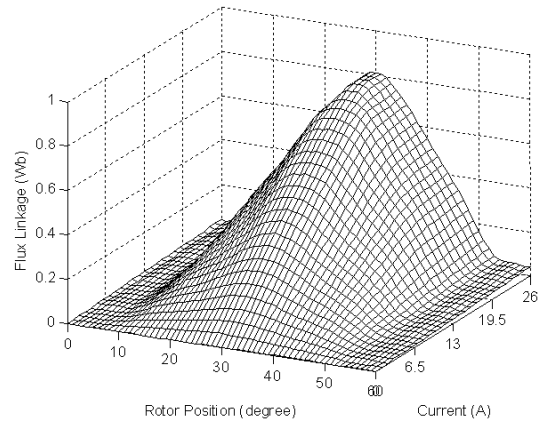
(a) Flux linkage
