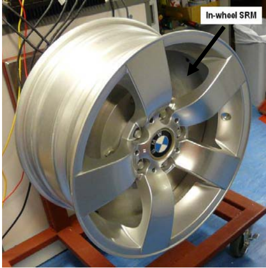
Fig. 3 Prototype of the in-wheel SRM
