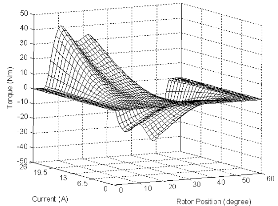
(b) Torque
