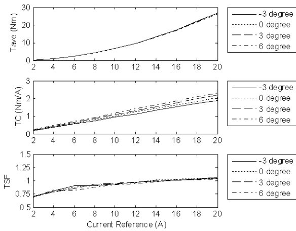
(c) Various turn-on angles
