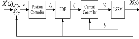
Fig.2 Block diagram for the structure of whole control system
