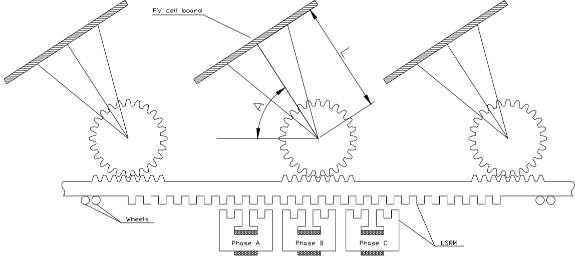
Fig.1 The design schematic of linear switched reluctance motor based solar tracking system
