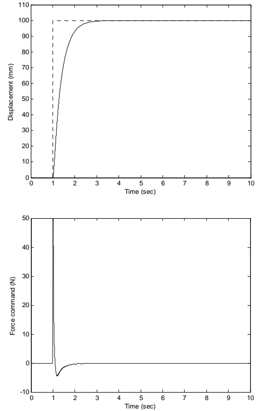
Fig.3 Simulation: step response and control signal waveform
